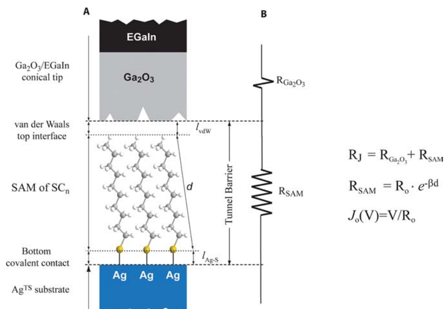
Figure 2. (A) Structure of Ag TS -SAM//Ga 2 O 3 /EGaIn junctions. (B) Components of the resistance of the junction ( R_J ): R_{SAM} , tunneling resistance across the SAM; R_{Ga_2O_3} , resistance of the Ga 2 O 3 layer; l_{Ag-S} , length of the bottom Ag TS -S covalent contact; l_{vdW} , thickness of the top SAM//Ga 2 O 3 van der Waals interface; d , length of the tunnel barrier established by the alkyl chain. Assuming a through-bond mechanism, d coincides with the length of the alkyl chain. J_0 is defined as the current across a junction with d = 0 .
